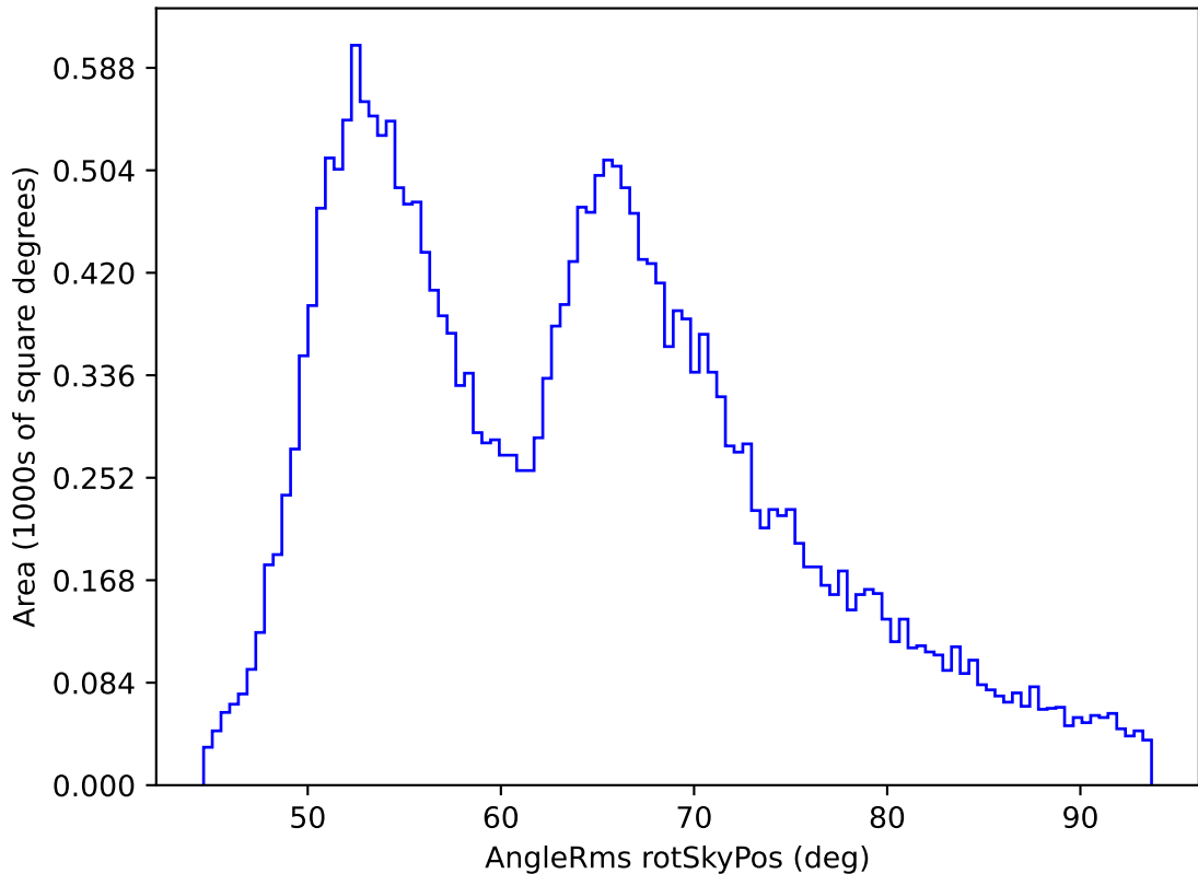
no_magell_roll_v3.4_10yrs All sky all bands: AngleRms rotSkyPos
