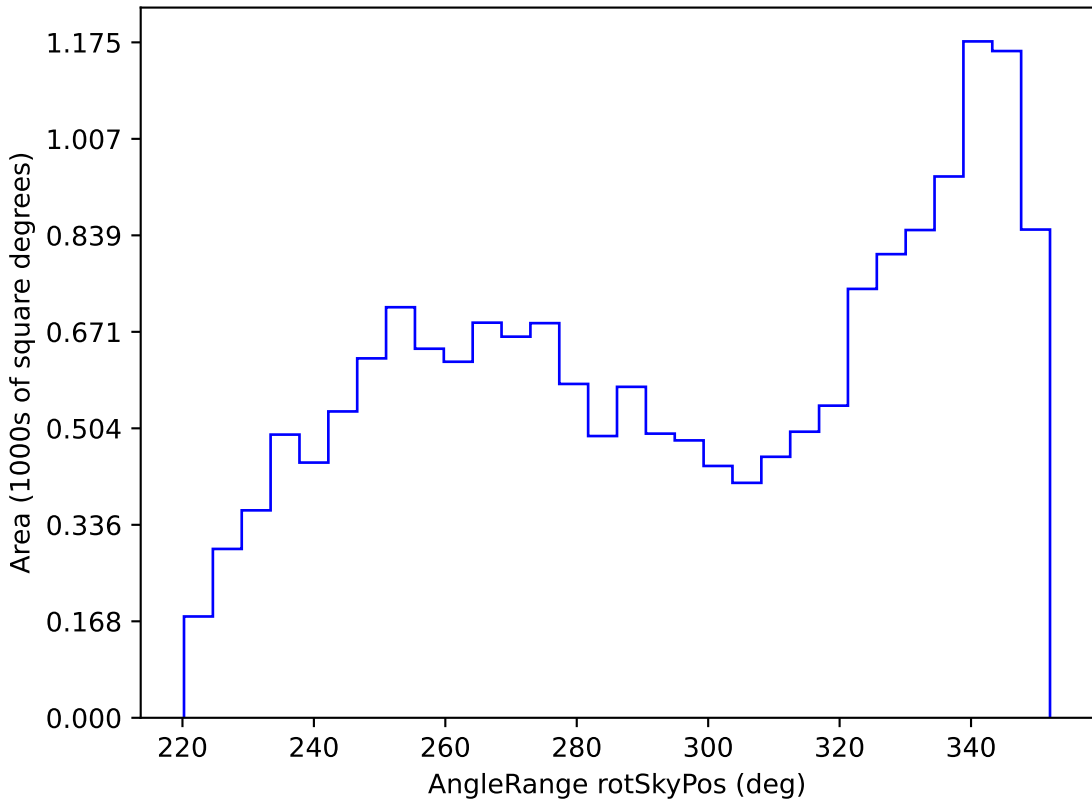
no_magell_roll_v3.4_10yrs WFD all bands: AngleRange rotSkyPos
