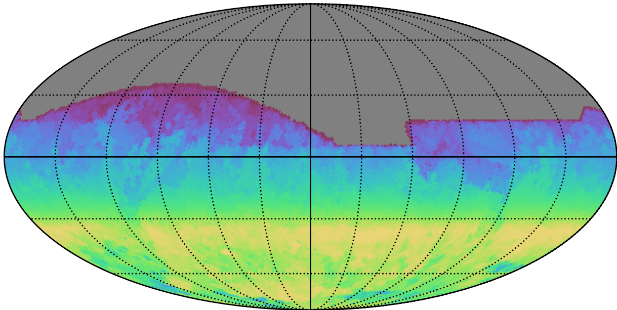
no_magell_roll_v3.4_10yrs All sky all bands: AngleRange rotSkyPos
