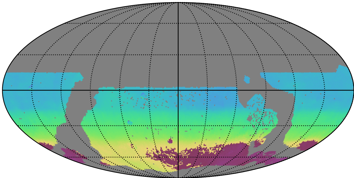
no_magell_roll_v3.4_10yrs WFD all bands: AngleMean rotSkyPos
