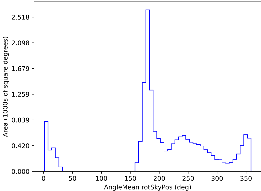
no_magell_roll_v3.4_10yrs WFD all bands: AngleMean rotSkyPos
