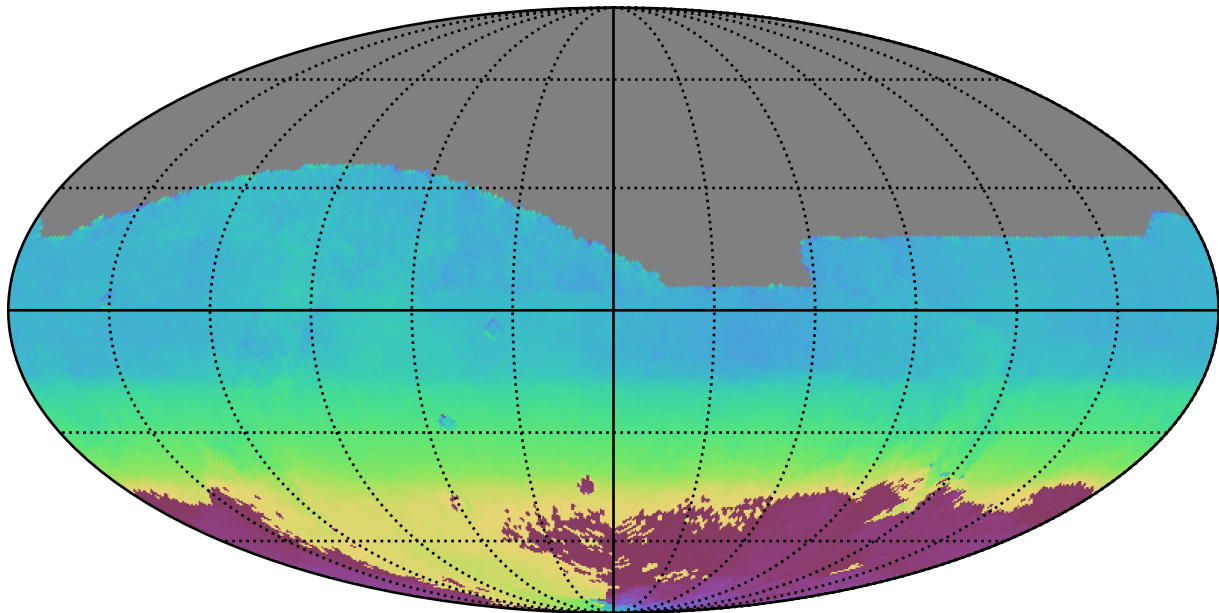
no_magell_roll_v3.4_10yrs All sky all bands: AngleMean rotSkyPos
