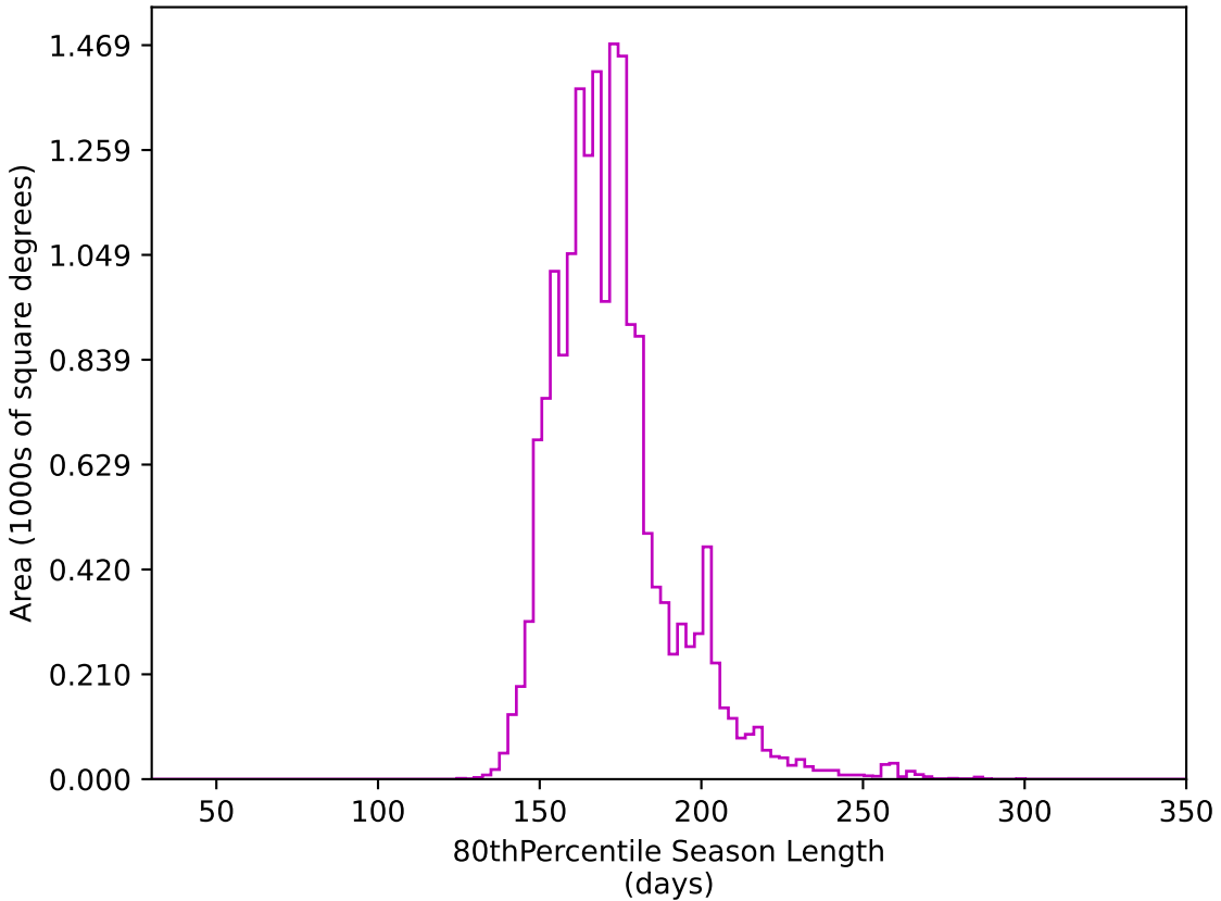
no_magell_roll_v3.4_10yrs WFD z band: 80thPercentile Season Length
