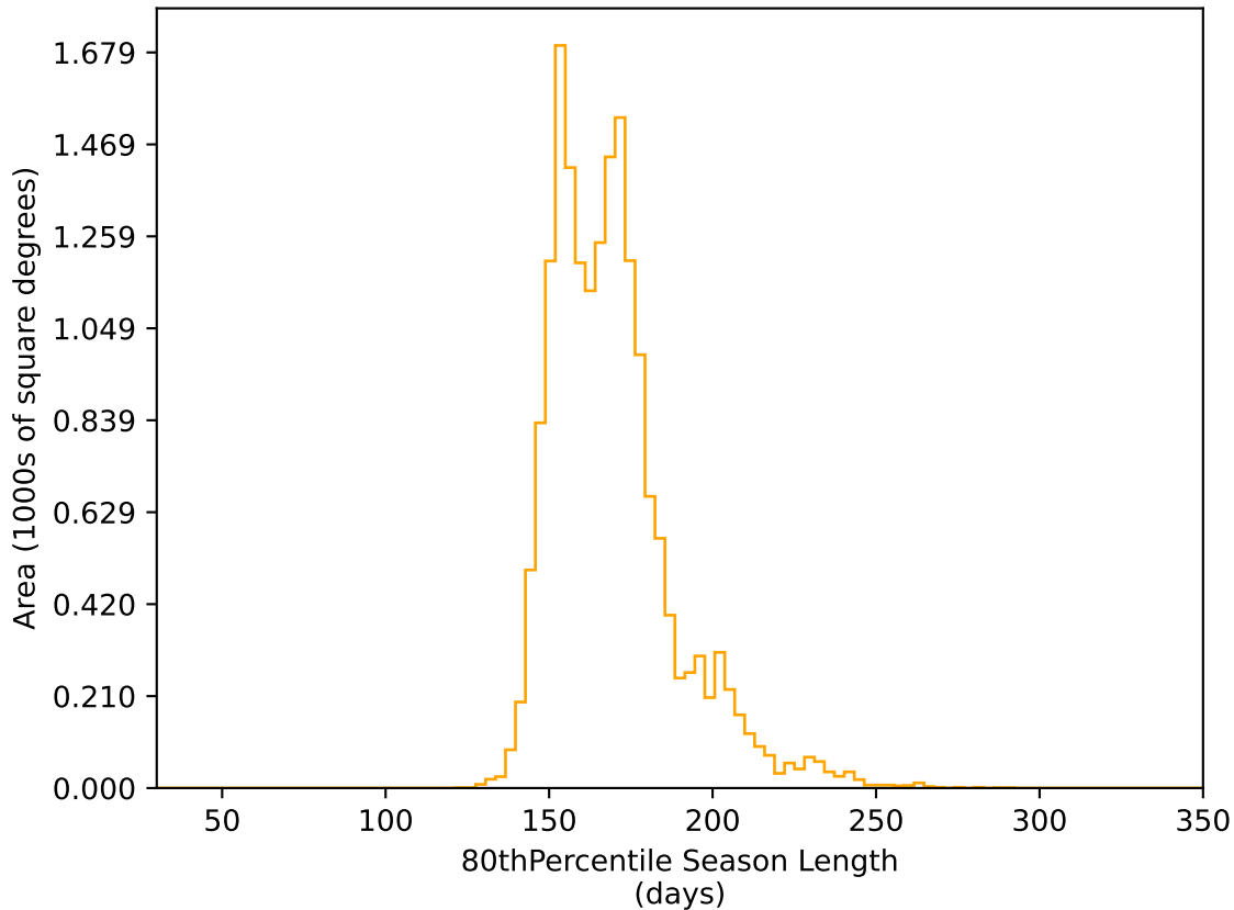
no_magell_roll_v3.4_10yrs WFD r band: 80thPercentile Season Length
