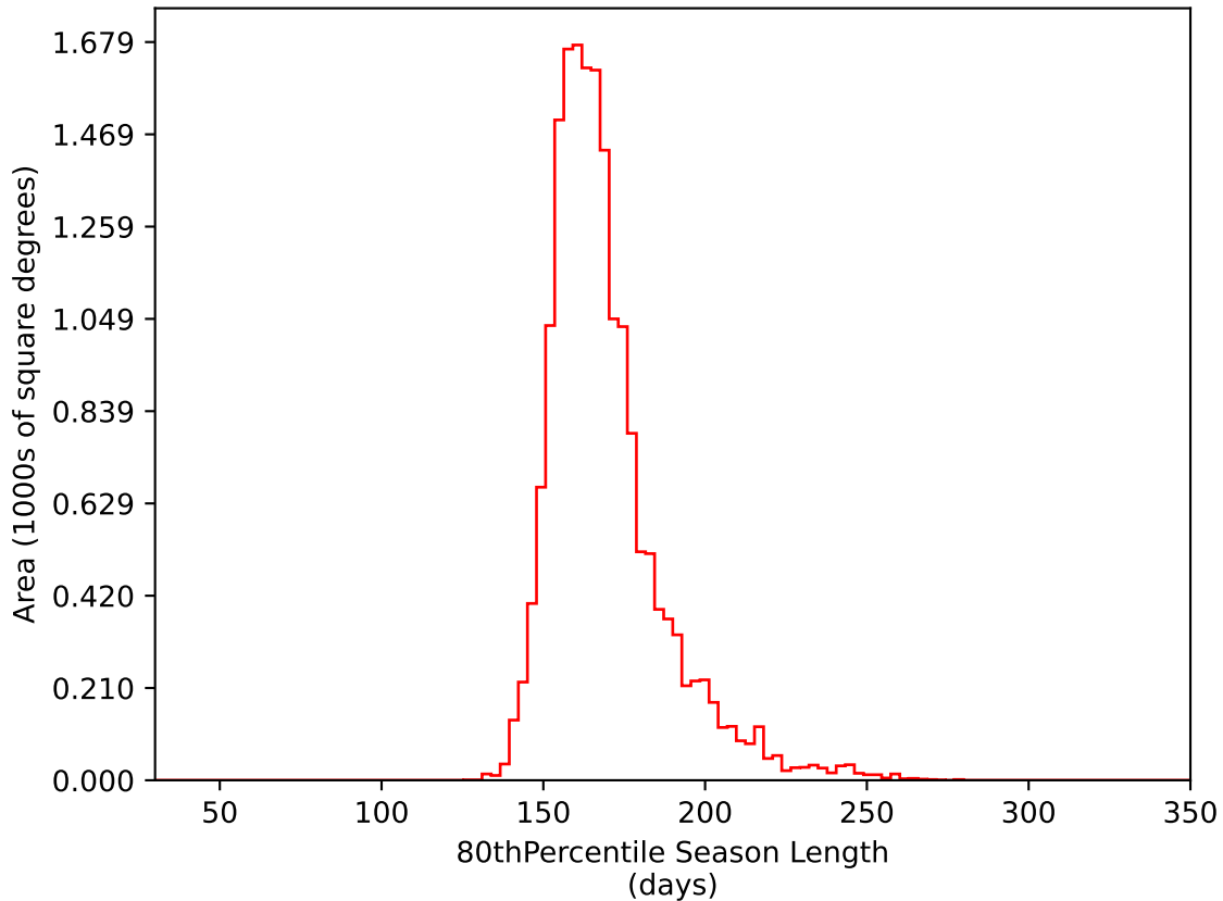
no_magell_roll_v3.4_10yrs WFD i band: 80thPercentile Season Length
