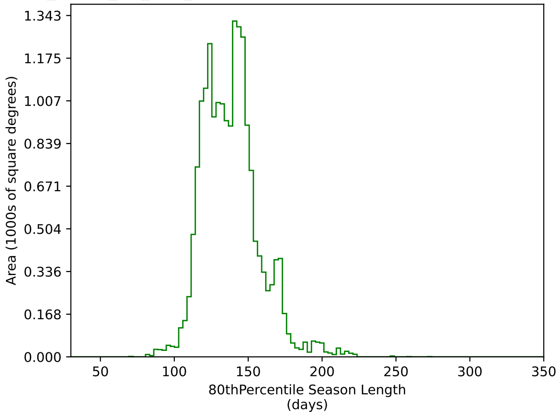
no_magell_roll_v3.4_10yrs WFD g band: 80thPercentile Season Length
