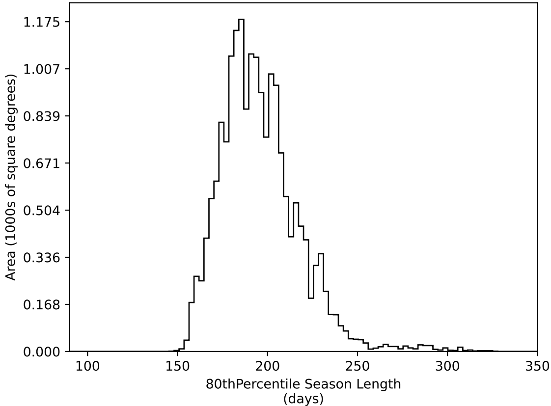
no_magell_roll_v3.4_10yrs WFD all bands: 80thPercentile Season Length
