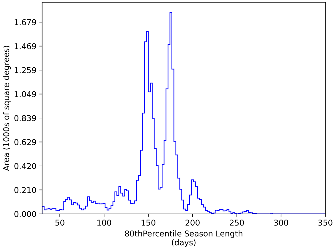
no_magell_roll_v3.4_10yrs All sky y band: 80thPercentile Season Length
