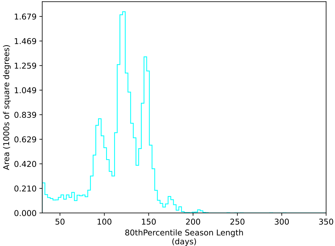
no_magell_roll_v3.4_10yrs All sky u band: 80thPercentile Season Length
