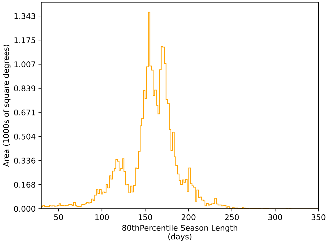
no_magell_roll_v3.4_10yrs All sky r band: 80thPercentile Season Length
