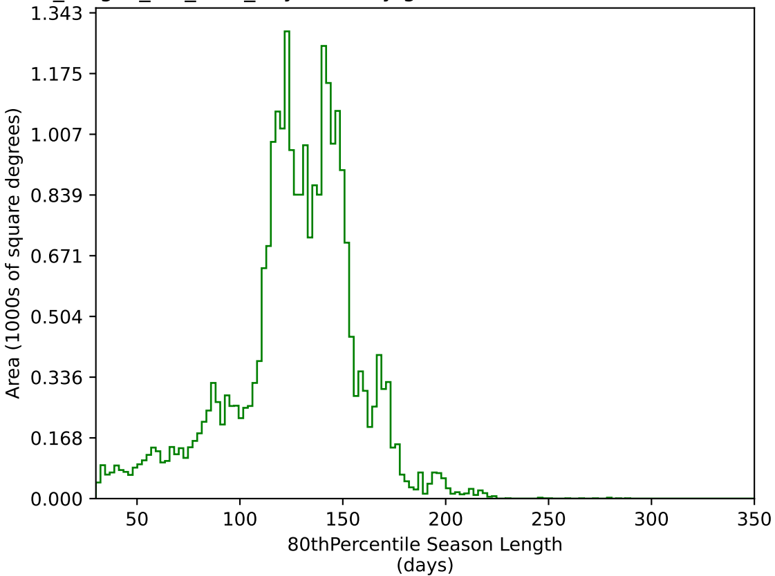
no_magell_roll_v3.4_10yrs All sky g band: 80thPercentile Season Length
