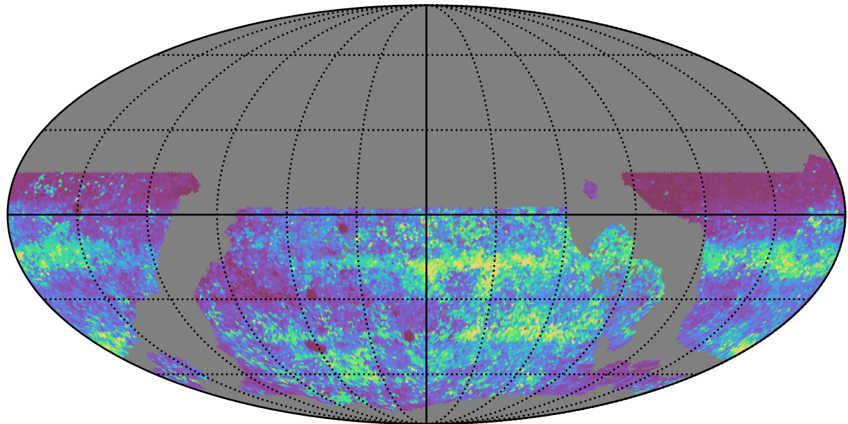
no_magell_roll_v3.4_10yrs WFD zy bands: 75th Percentile Intranight Timespan
