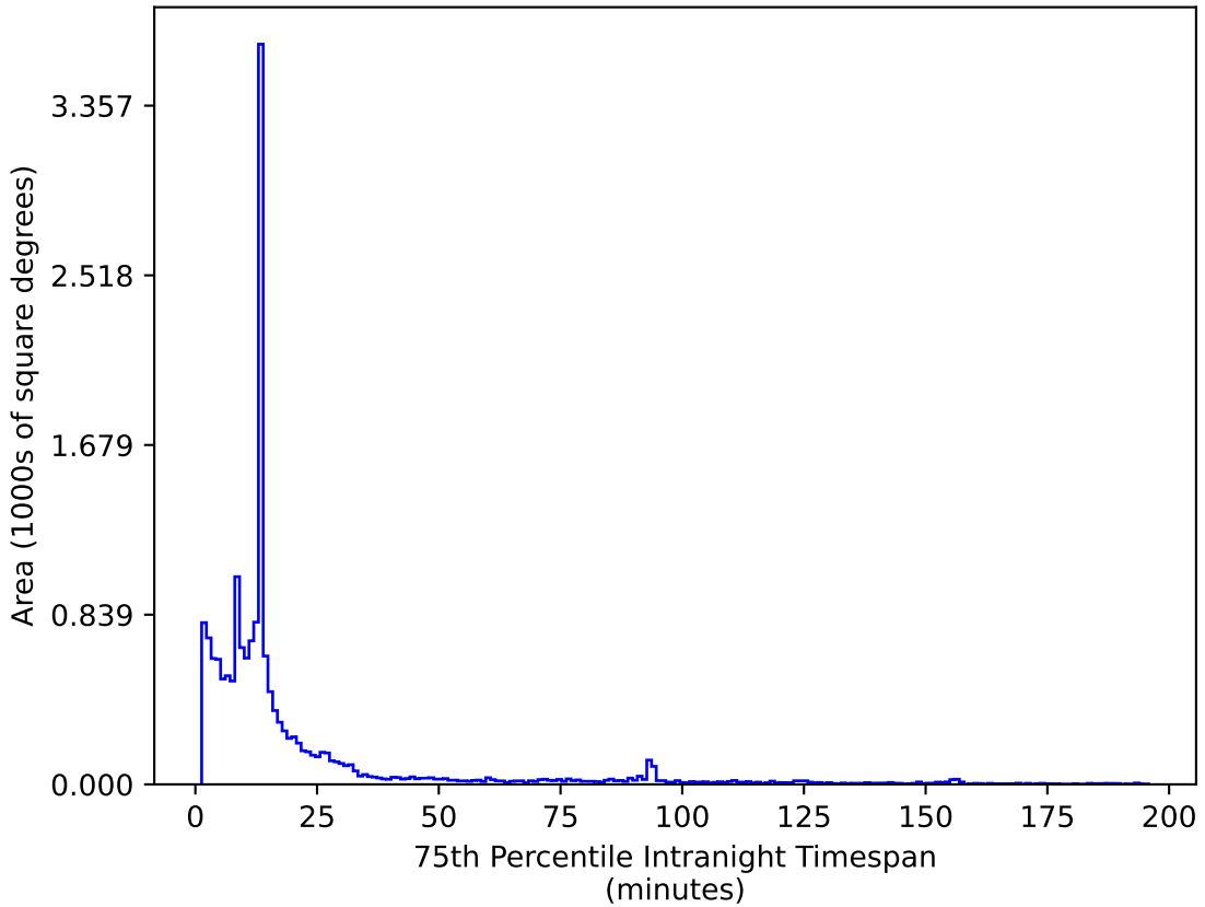
no_magell_roll_v3.4_10yrs WFD z band: 75th Percentile Intranight Timespan
