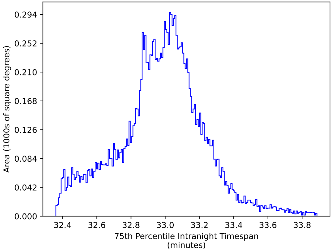
no_magell_roll_v3.4_10yrs WFD y band: 75th Percentile Intranight Timespan
