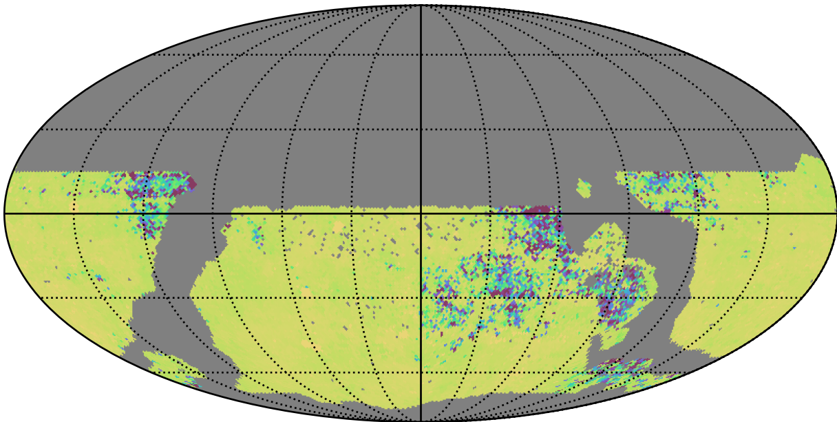
no_magell_roll_v3.4_10yrs WFD ug bands: 75th Percentile Intranight Timespan
