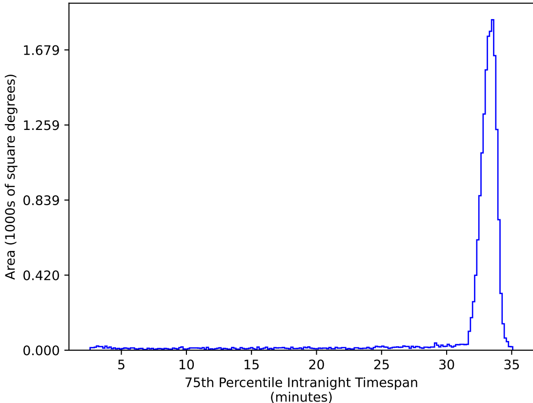
no_magell_roll_v3.4_10yrs WFD ug bands: 75th Percentile Intranight Timespan
