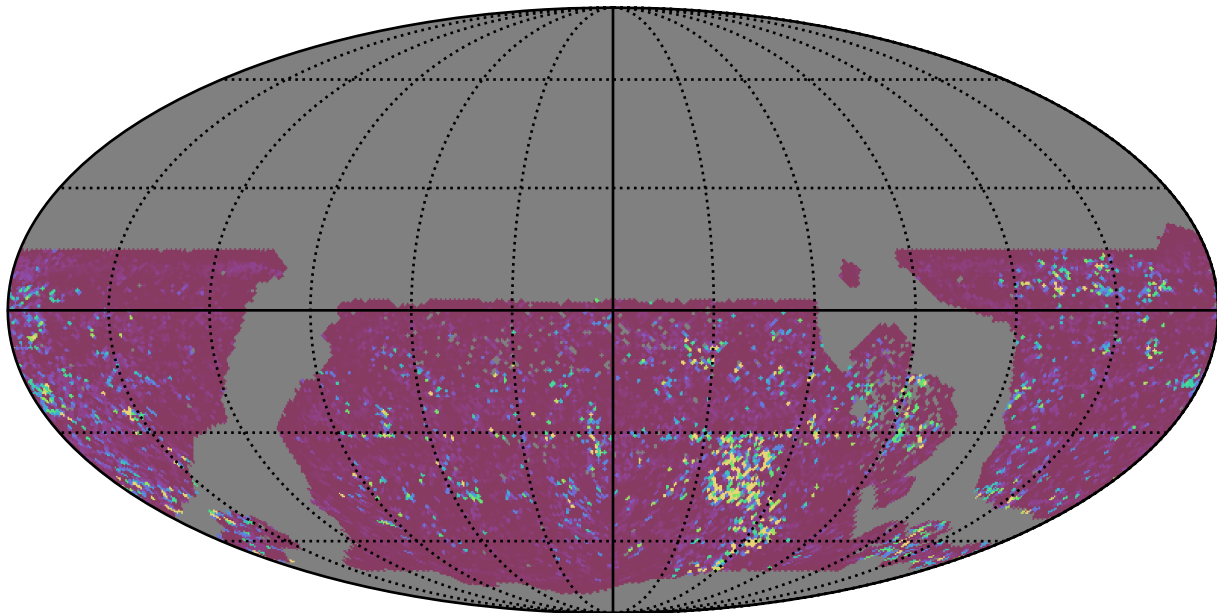
no_magell_roll_v3.4_10yrs WFD u band: 75th Percentile Intranight Timespan
