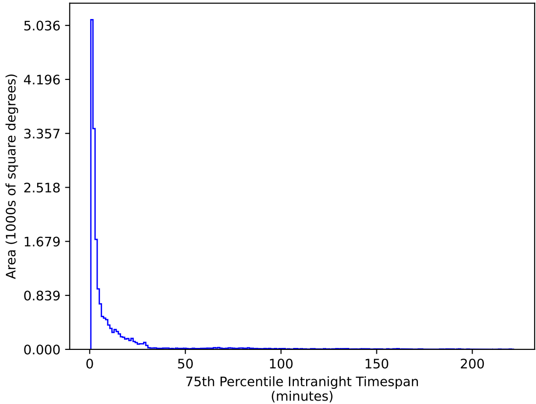
no_magell_roll_v3.4_10yrs WFD u band: 75th Percentile Intranight Timespan
