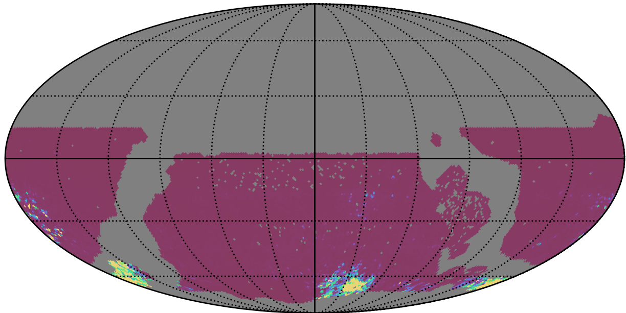
no_magell_roll_v3.4_10yrs WFD ri bands: 75th Percentile Intranight Timespan
