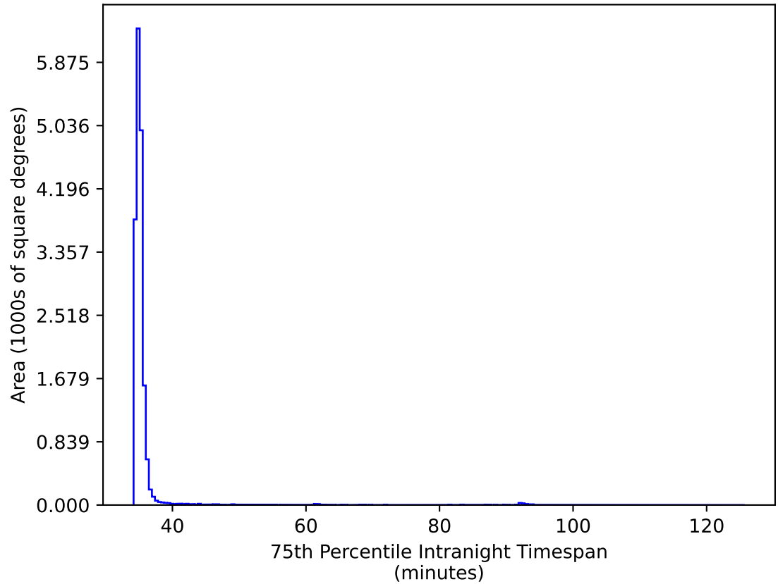
no_magell_roll_v3.4_10yrs WFD ri bands: 75th Percentile Intranight Timespan
