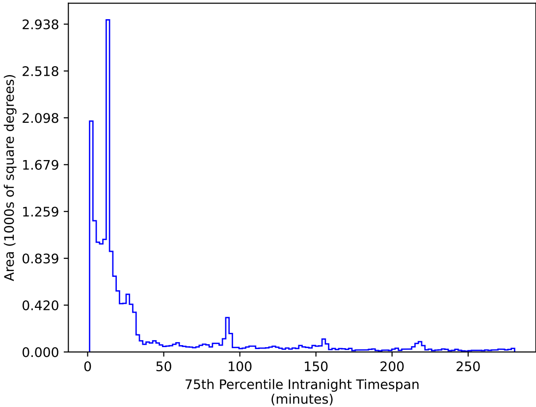
no_magell_roll_v3.4_10yrs WFD r band: 75th Percentile Intranight Timespan
