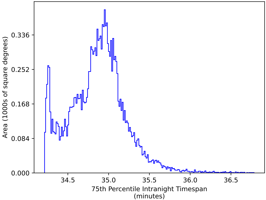
no_magell_roll_v3.4_10yrs WFD iz bands: 75th Percentile Intranight Timespan
