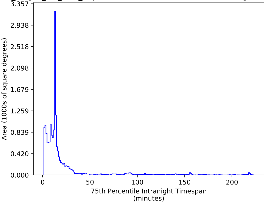
no_magell_roll_v3.4_10yrs WFD i band: 75th Percentile Intranight Timespan
