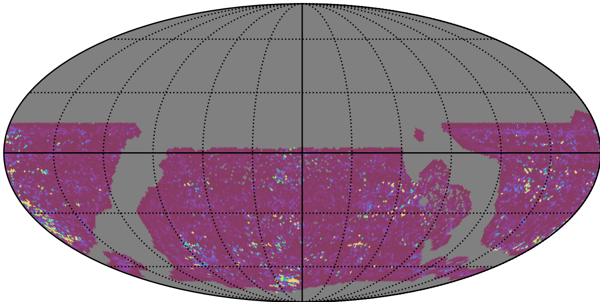
no_magell_roll_v3.4_10yrs WFD g band: 75th Percentile Intranight Timespan
