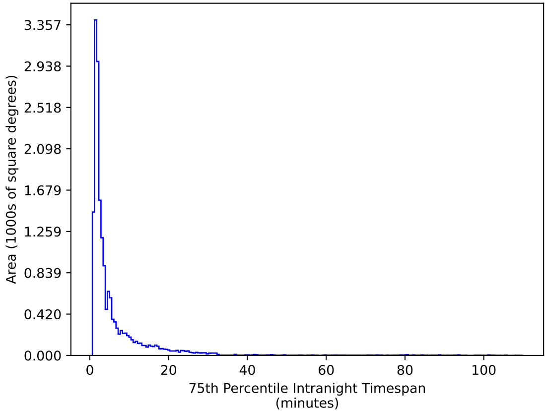
no_magell_roll_v3.4_10yrs WFD g band: 75th Percentile Intranight Timespan
