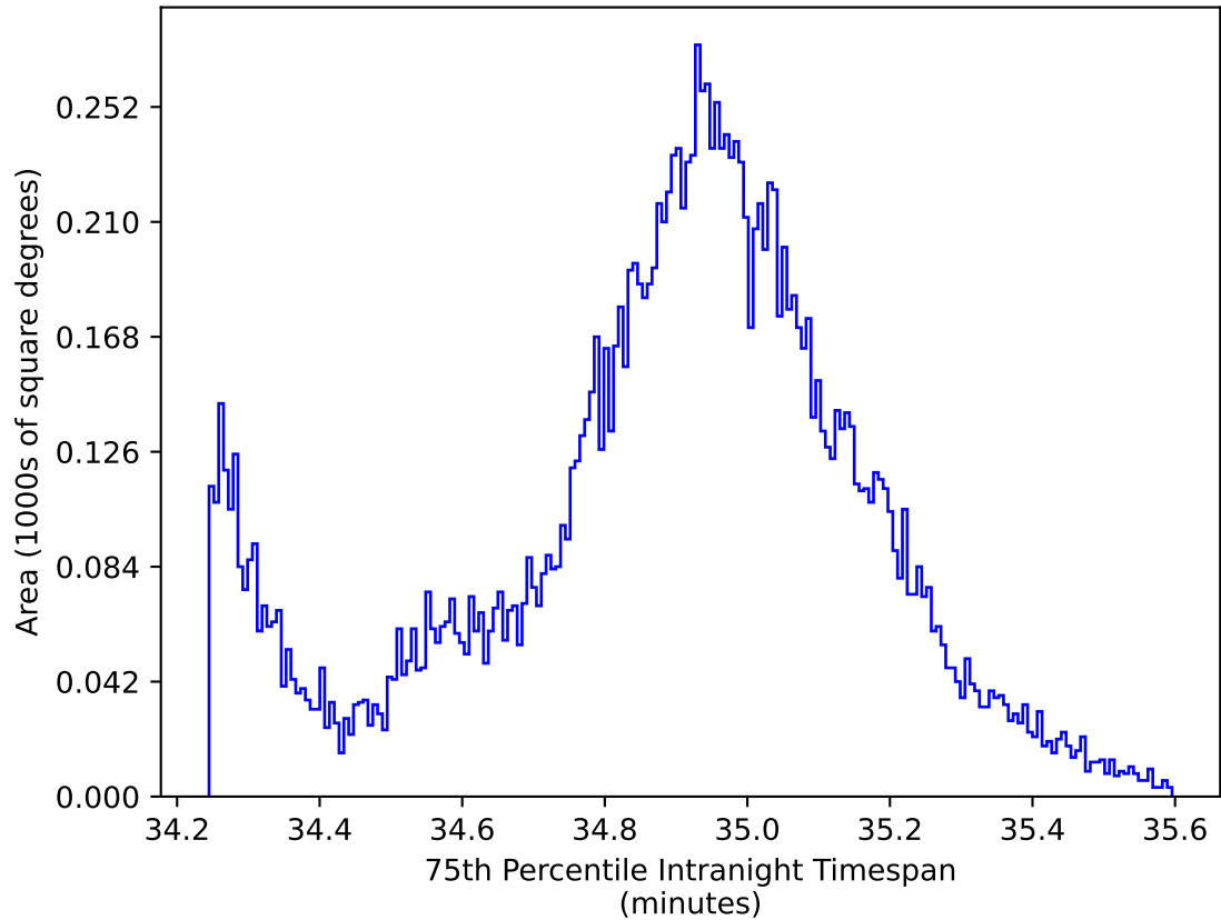
no_magell_roll_v3.4_10yrs WFD all bands: 75th Percentile Intranight Timespan
