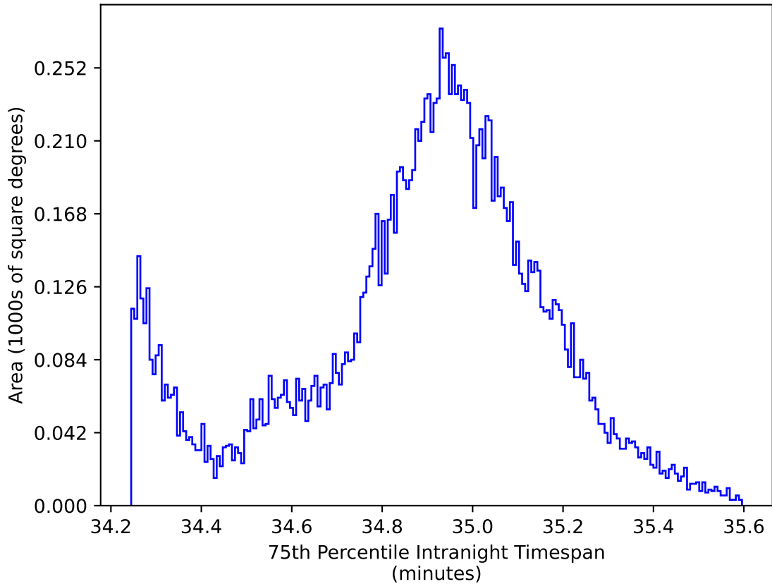
no_magell_roll_v3.4_10yrs WFD: 75th Percentile Intranight Timespan
