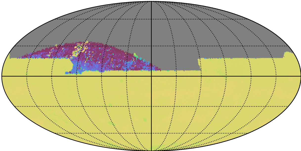
no_magell_roll_v3.4_10yrs All sky zy bands: 75th Percentile Intranight Timespan
