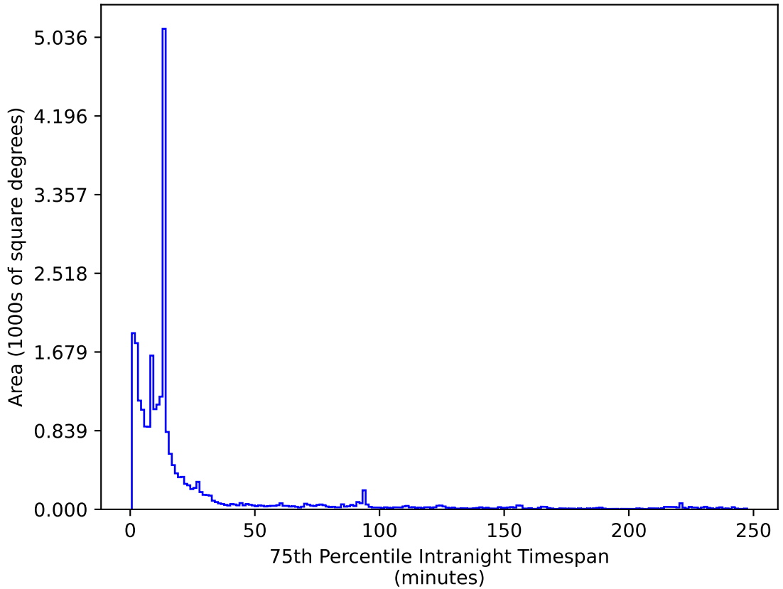
no_magell_roll_v3.4_10yrs All sky z band: 75th Percentile Intranight Timespan
