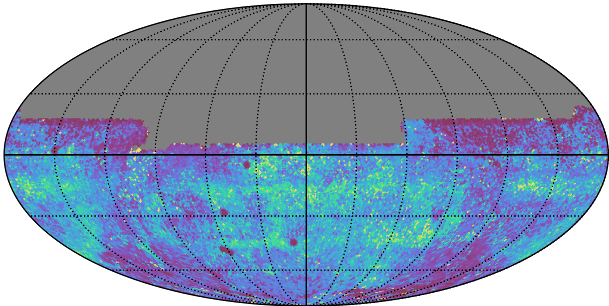
no_magell_roll_v3.4_10yrs All sky y band: 75th Percentile Intranight Timespan
