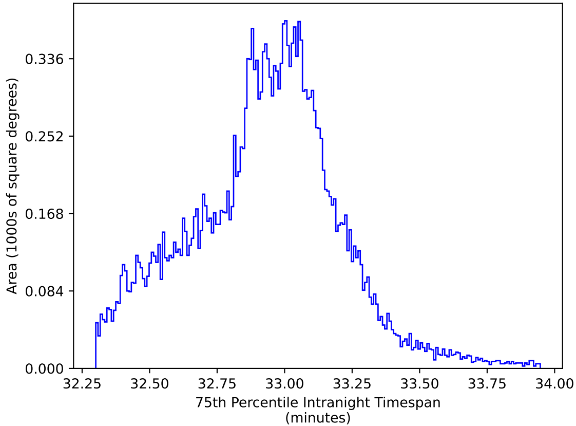
no_magell_roll_v3.4_10yrs All sky y band: 75th Percentile Intranight Timespan
