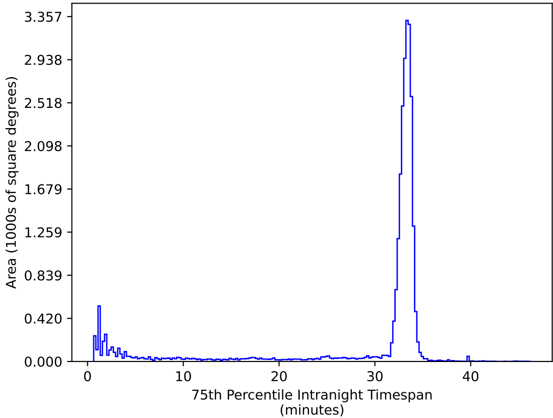
no_magell_roll_v3.4_10yrs All sky ug bands: 75th Percentile Intranight Timespan
