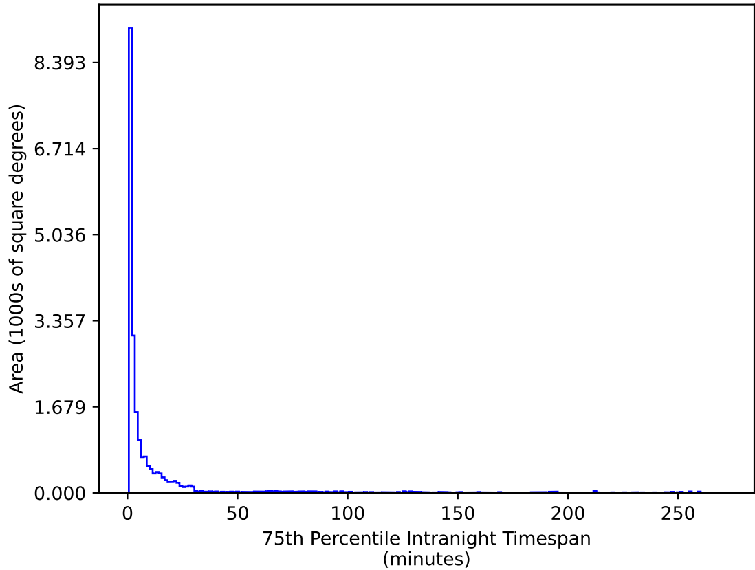
no_magell_roll_v3.4_10yrs All sky u band: 75th Percentile Intranight Timespan
