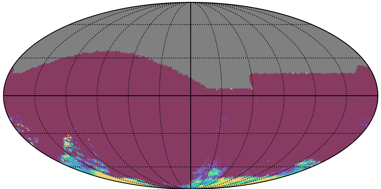
no_magell_roll_v3.4_10yrs All sky ri bands: 75th Percentile Intranight Timespan
