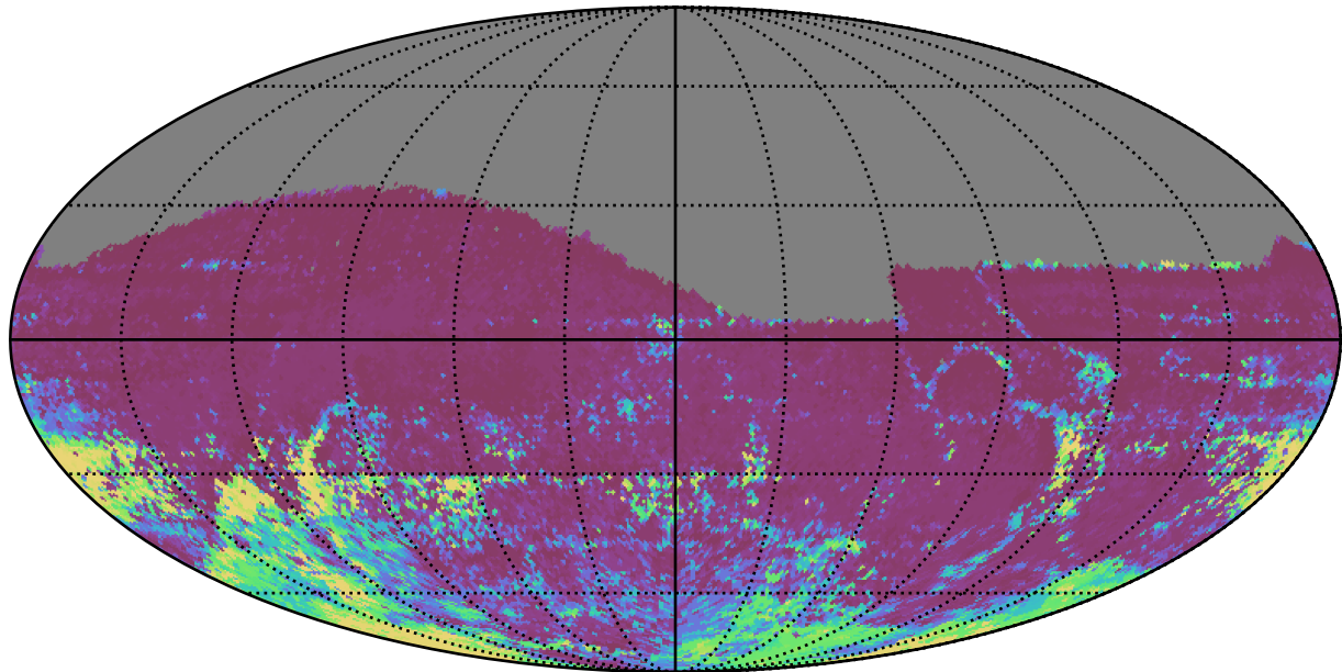
no_magell_roll_v3.4_10yrs All sky r band: 75th Percentile Intranight Timespan
