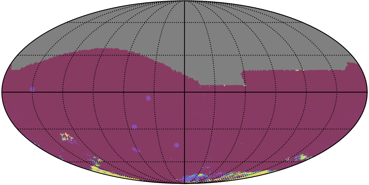
no_magell_roll_v3.4_10yrs All sky iz bands: 75th Percentile Intranight Timespan
