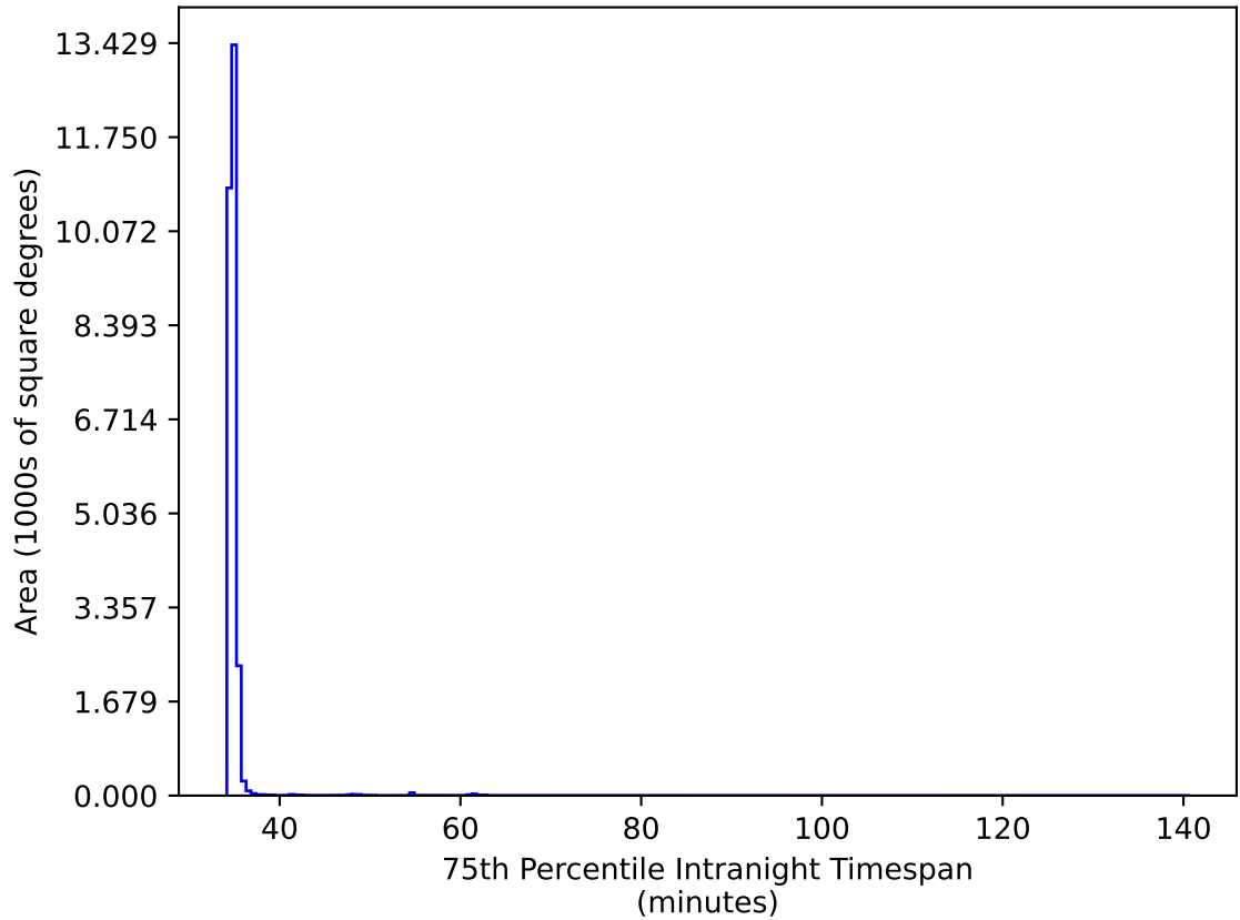
no_magell_roll_v3.4_10yrs All sky iz bands: 75th Percentile Intranight Timespan
