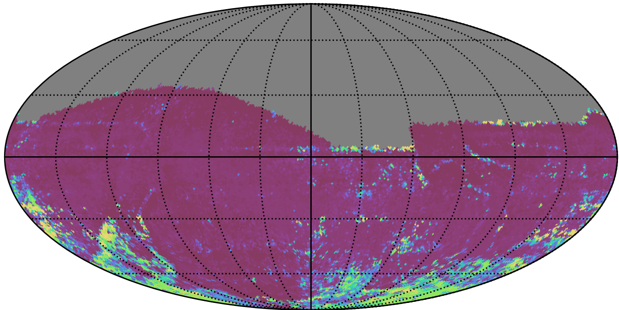
no_magell_roll_v3.4_10yrs All sky i band: 75th Percentile Intranight Timespan
