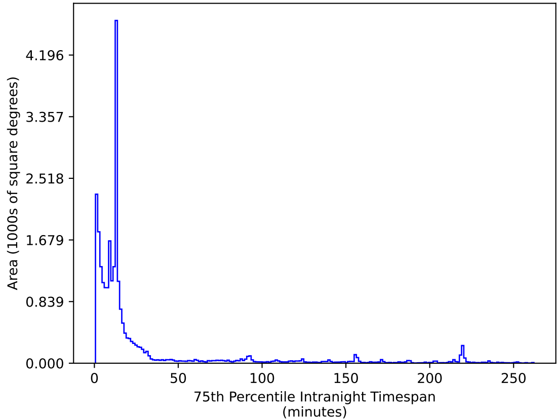
no_magell_roll_v3.4_10yrs All sky i band: 75th Percentile Intranight Timespan
