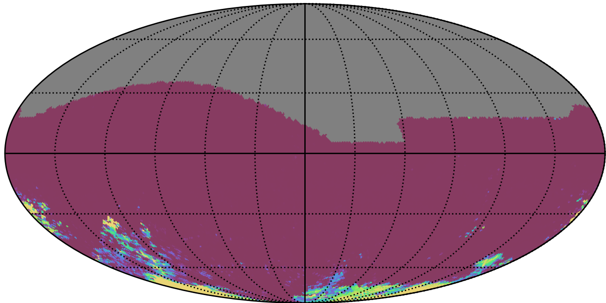
no_magell_roll_v3.4_10yrs All sky gr bands: 75th Percentile Intranight Timespan
