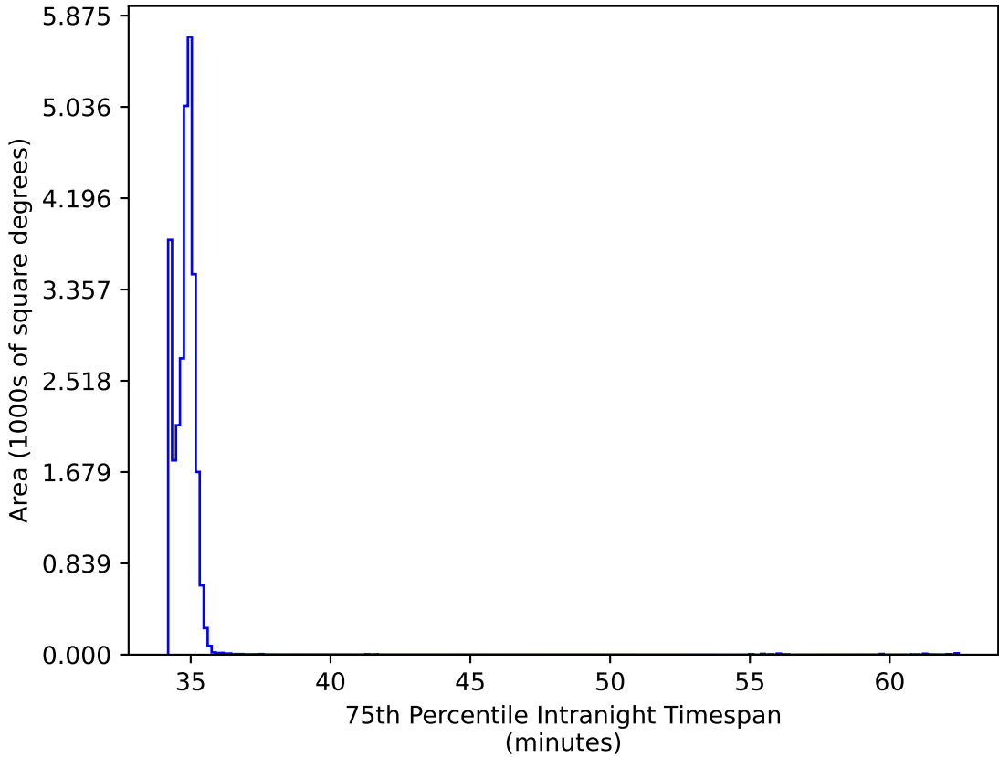
no_magell_roll_v3.4_10yrs All sky all bands: 75th Percentile Intranight Timespan
