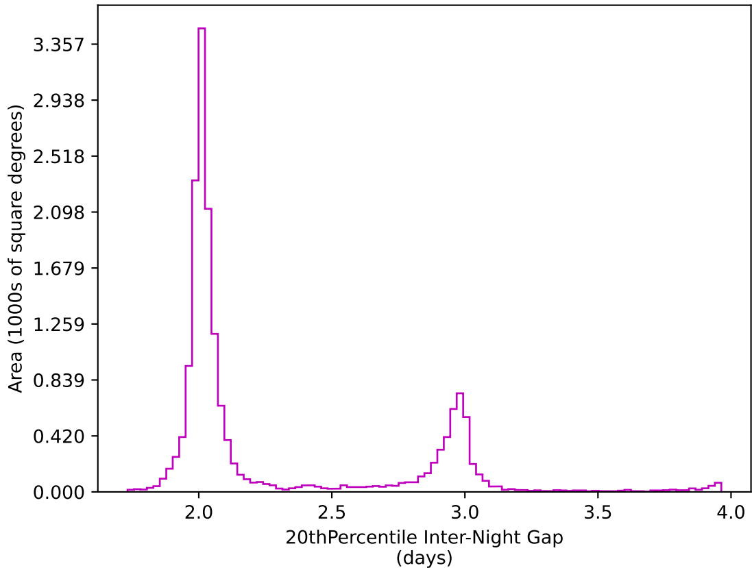
no_magell_roll_v3.4_10yrs WFD z band: 20thPercentile Inter-Night Gap
