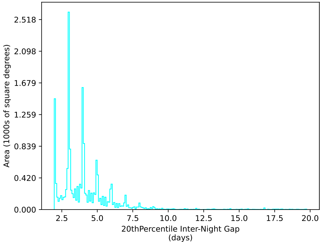
no_magell_roll_v3.4_10yrs WFD u band: 20thPercentile Inter-Night Gap
