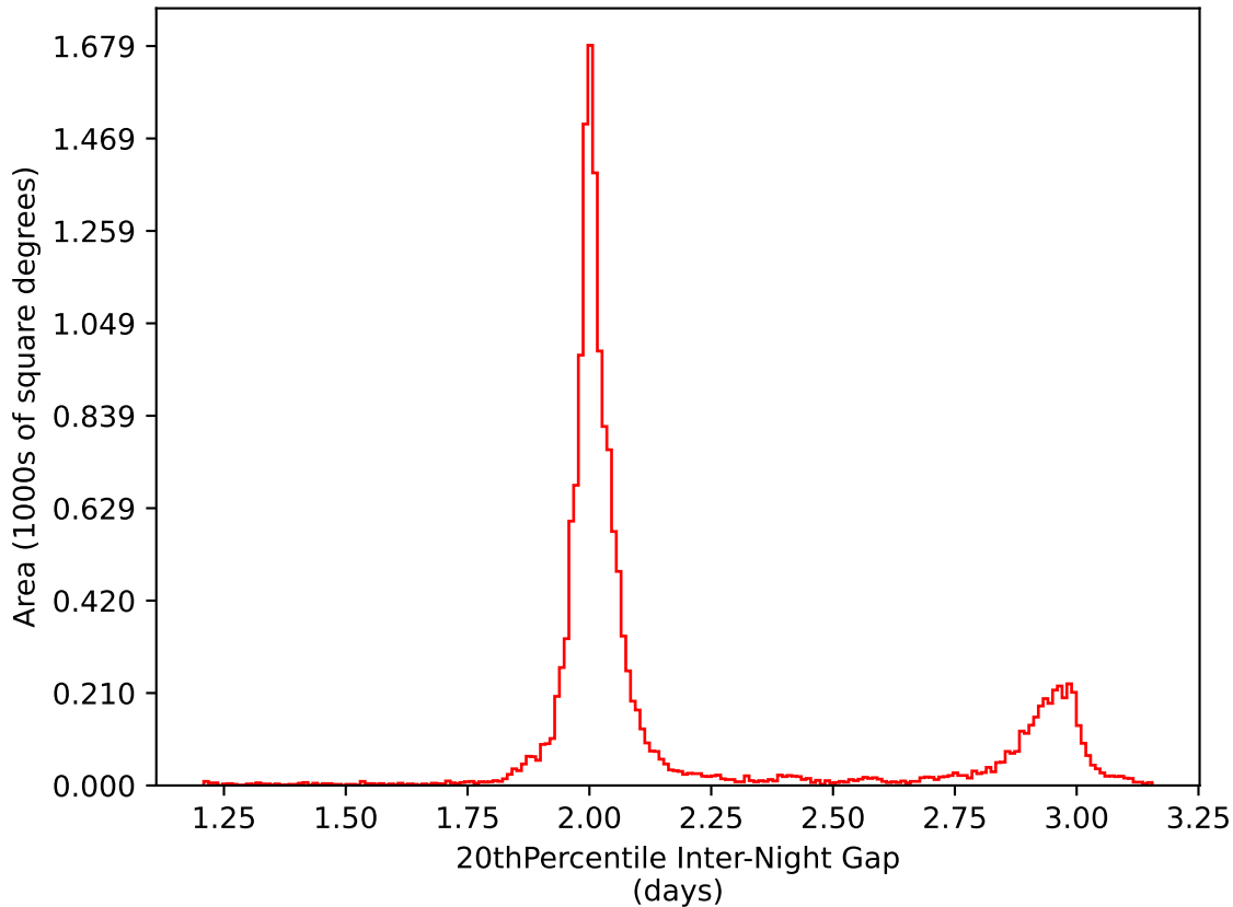
no_magell_roll_v3.4_10yrs WFD i band: 20thPercentile Inter-Night Gap
