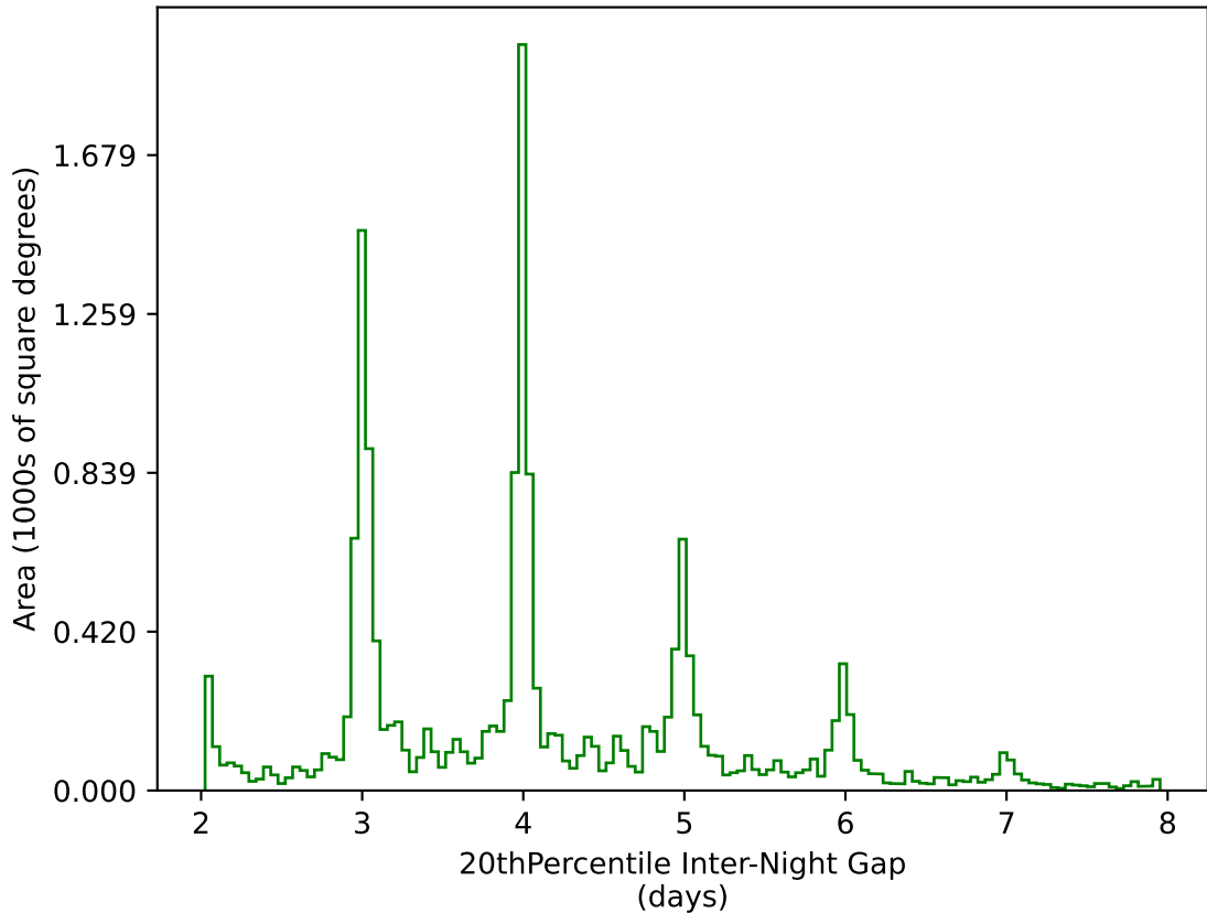
no_magell_roll_v3.4_10yrs WFD g band: 20thPercentile Inter-Night Gap
