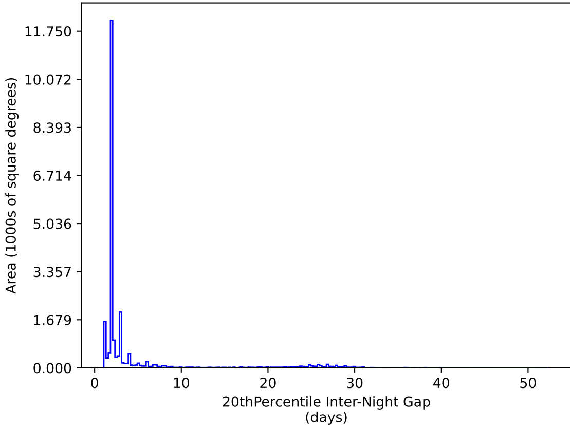
no_magell_roll_v3.4_10yrs All sky y band: 20thPercentile Inter-Night Gap
